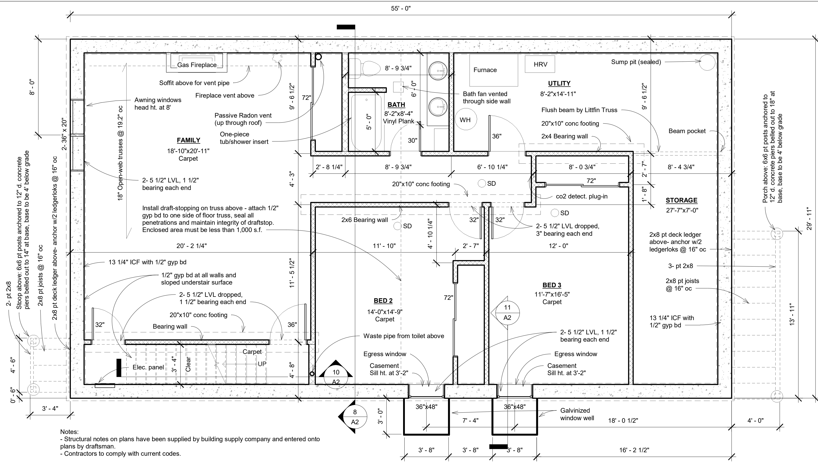
1 Lower Level 1/4" = 1'-0"
