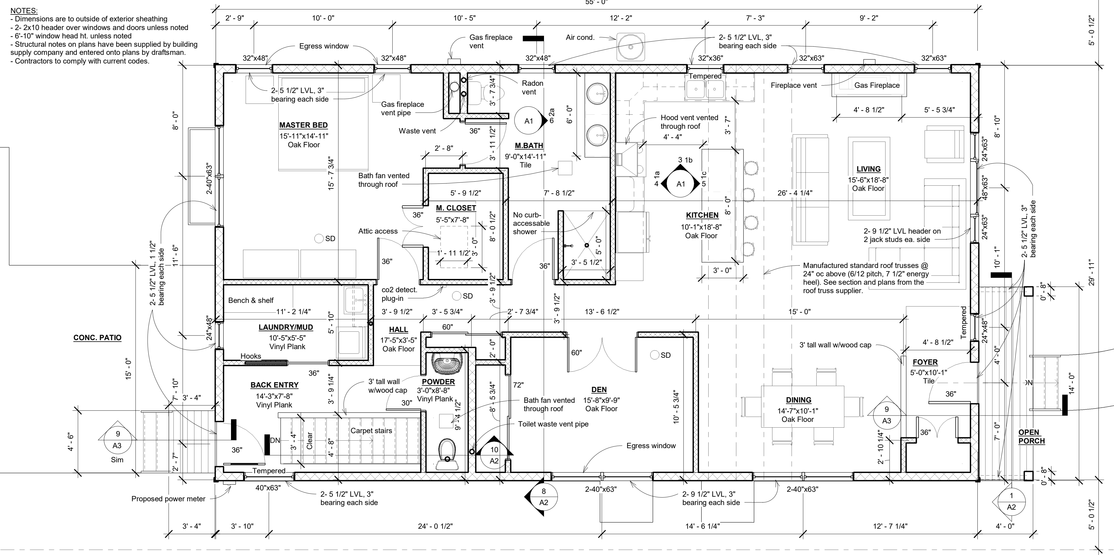
2 Main Level 1/4" = 1'-0"
