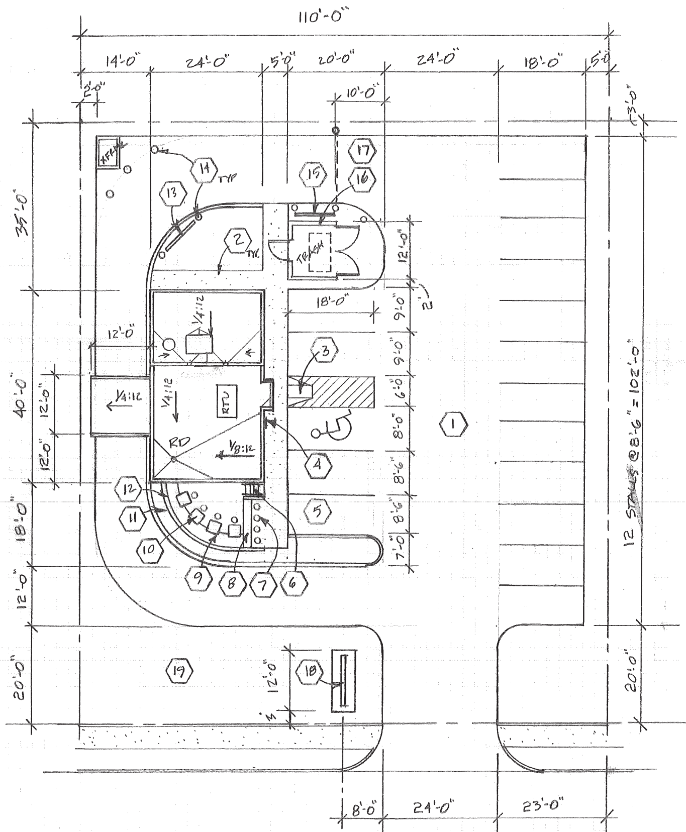
SITE PLAN 1"=20'
